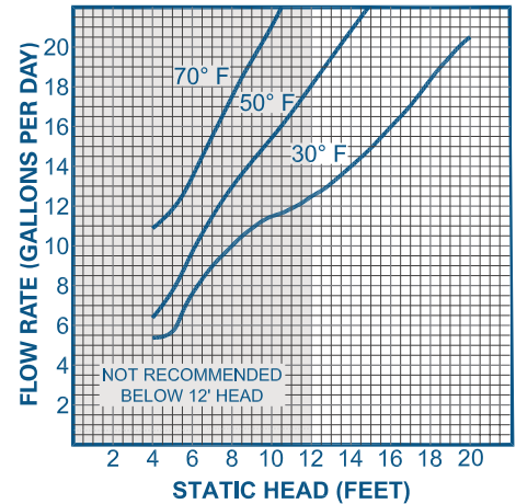
30 WT. OIL FLOW CHARACTERISTICS
