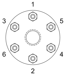
Recommended Nut Tightening Sequence
