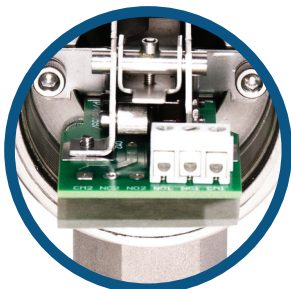
Terminal Block
