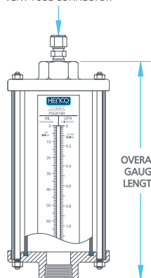
FNPT INLET PORT GAUGE WITH 316 S.S. END PLATES
