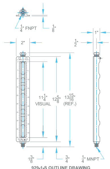
929-1-S OUTLINE DRAWING
