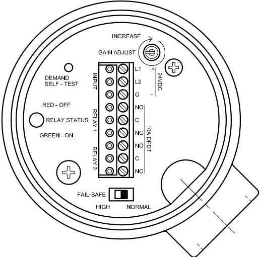
10A DPDT OUTPUT ELECTRONICS MODULE
