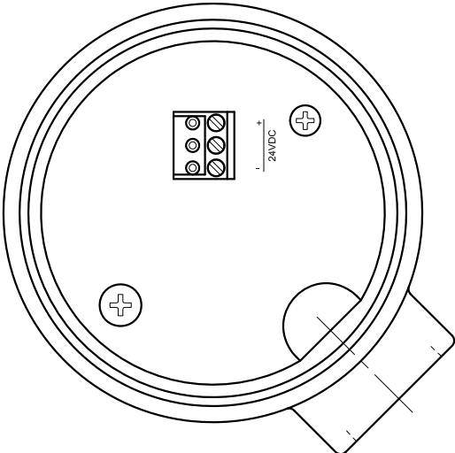
4-20mA OUTPUT ELECTRONICS MODULE
